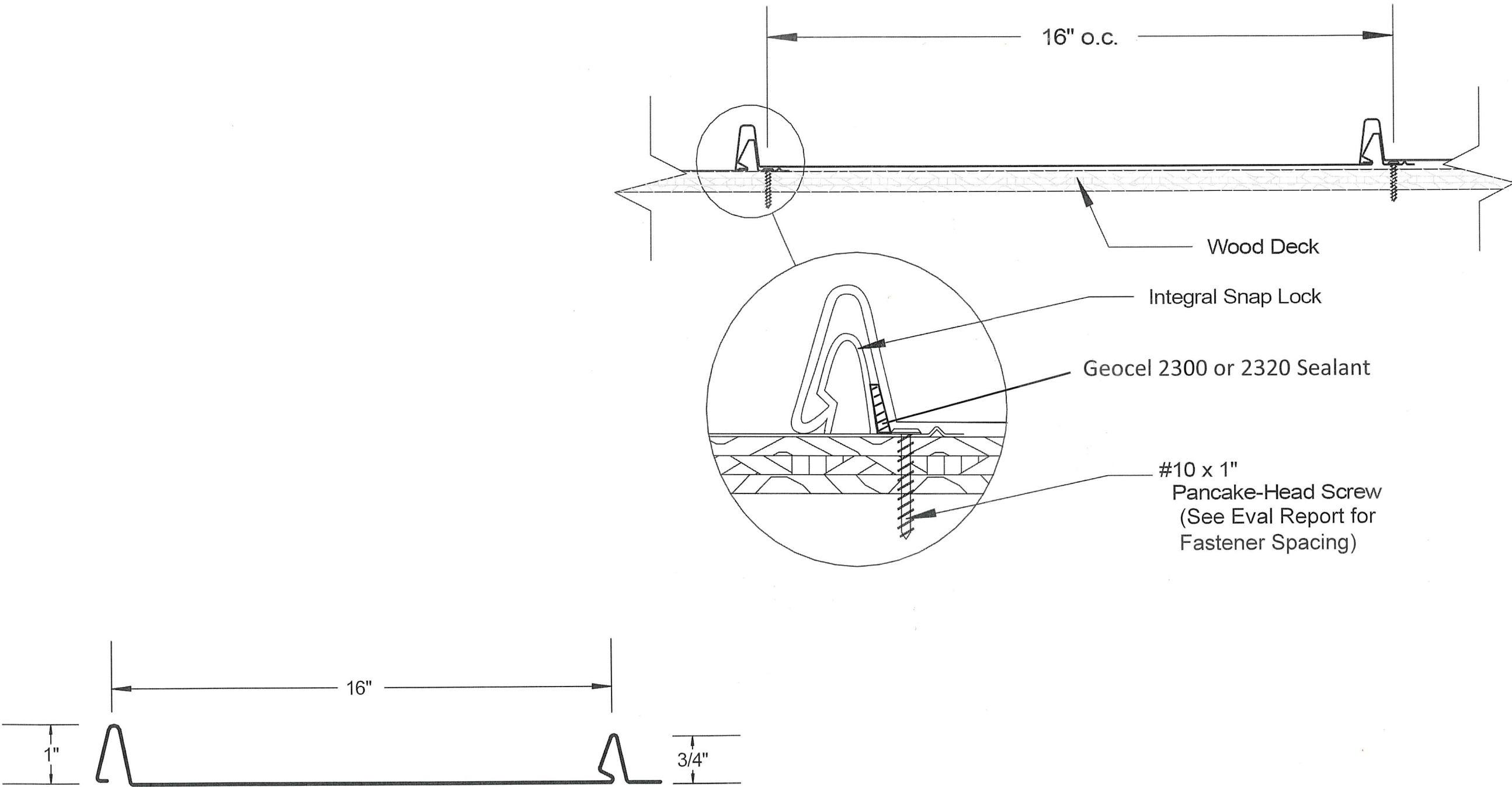
Panel Profile
